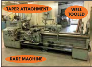
AMERICAN "STYLE - C" 16"x 78" ENGINE LATHE
