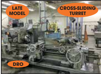
WARNER & SWASEY # 2A "Square Head" TURRET LATHE
