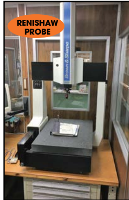
BROWN & SHARPE CMM w/ Cabinet Base
