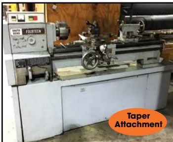
SOUTH-BEND 14"x 40" TOOL ROOM LATHE
