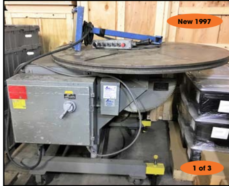
ARONSON #HD-25A WELDING POSITIONER
