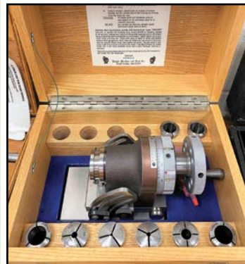
VIEW of (300+) HARIG - KNIGHT - PARLEC - MITUTOYO FIXTURE & INSPECTION ITEMS
