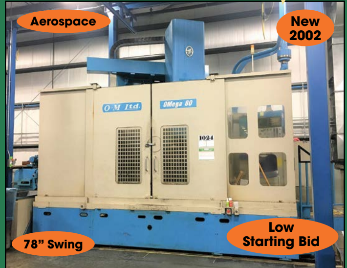
OM # OMEGA-80 (63" CHUCK) CNC VERTICAL TURNING CENTER
