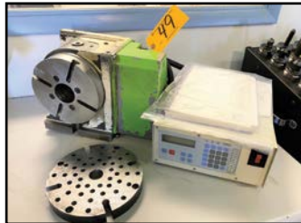
KOMA CNC "4th-Axis" ROTARY TABLE w/ Tsudakoma CNC Control
