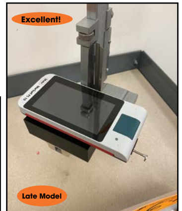
MAHR # MARSURF-PS-10 PROFILOMETER SURFACE TESTER
