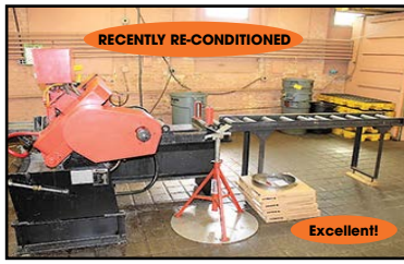
AMADA #HA-250W "AUTOMATIC" BAND SAW
