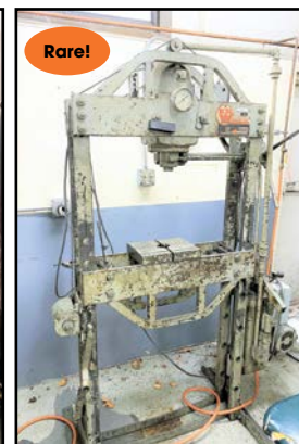
K.R. WILSON 50-Ton HYDRAULIC SHOP PRESS
