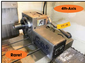
FADAL #VH-65 "4-AXIS" CNC ROTARY TABLE
