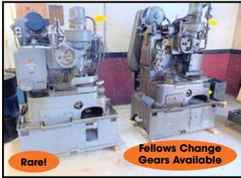
VIEW of FELLOWS GEAR SHAPERS
