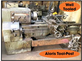
LEBLOND 17"x 54" ENGINE LATHE
