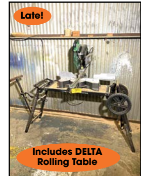
HITACHI COMPOUND CHOP SAW
