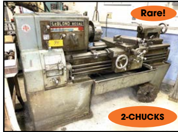
LEBLOND #REGAL 17" x 36" ENGINE LATHE
