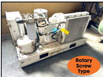
GARDNER-DENVER #EBE99K (30HP) AIR COMPRESSOR
